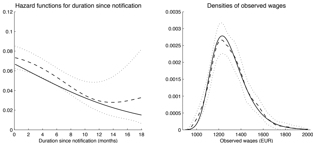
Figure 3: Goodness of Fit of the Model
