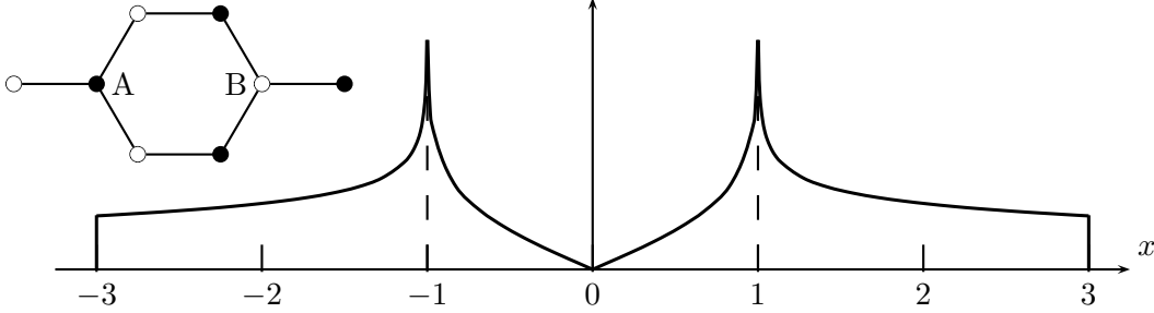
FIGURE 3. Graphene: nearest neighbors and density of states.
