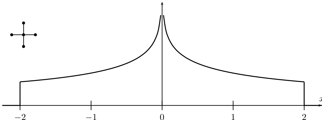
FIGURE 2. Square lattice: nearest neighbors and density of states.
