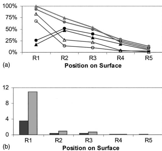
Fig. 4. A comparison of sputtered species with Xe and SF 5 at 5.0 keV as a function of the initial position on the surface. (a) Percentage of molecules at each surface position removed as yield (filled) or as damage (open). The total percentage of molecules removed is shown in gray. Circles represent values with Xe and triangles represent values with SF 5 . (b) Average number of total polystyrene fragments ejected.
