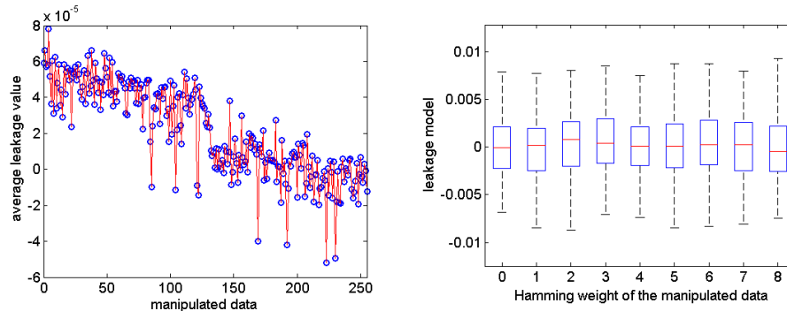
Fig. 2. 65nm S-box leakage model: avg. values (left) and grouped by HWs (right).
