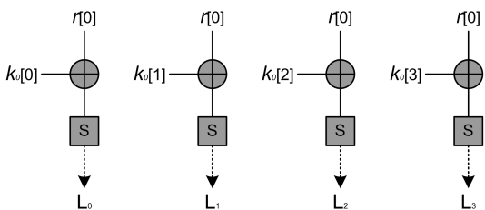
Fig. 3 Attacks against the first S-box layer.
