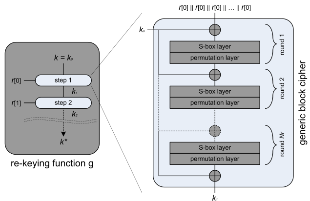
Fig. 2 Our instance of re-keying function g .
