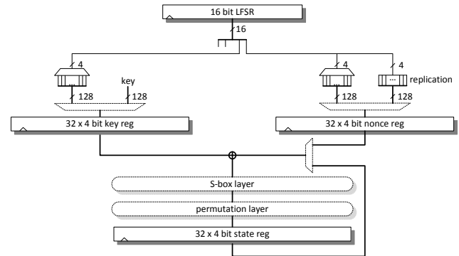
Fig. 7 Prototype architecture for worst-case EM profiling.
