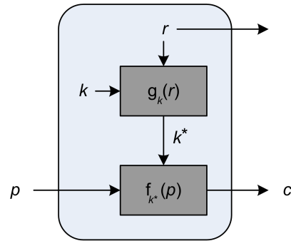
Fig. 1 Fresh re-keying: basic principle.
