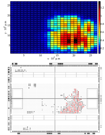
Fig. 5 Above: SNR over the 27 \times 27 chip surface. Below: Placement on the floorplan
