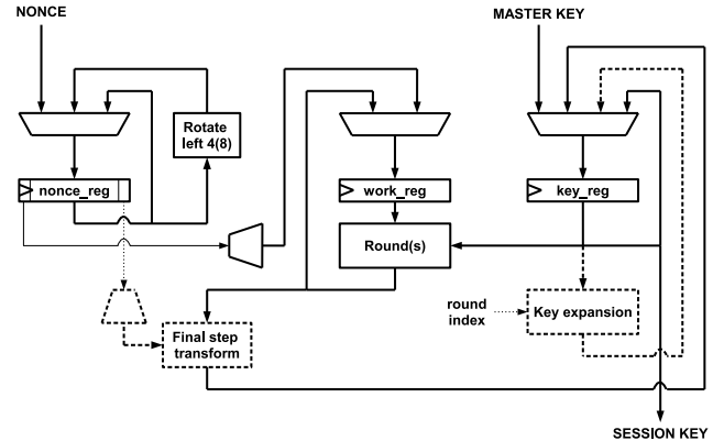
Fig. 6 Overview of our open source hardware architecture for fresh re-keying.
