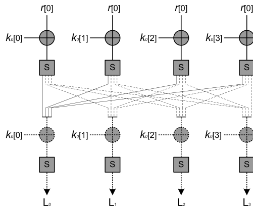
Fig. 4 Attacks against the second S-box layer.
