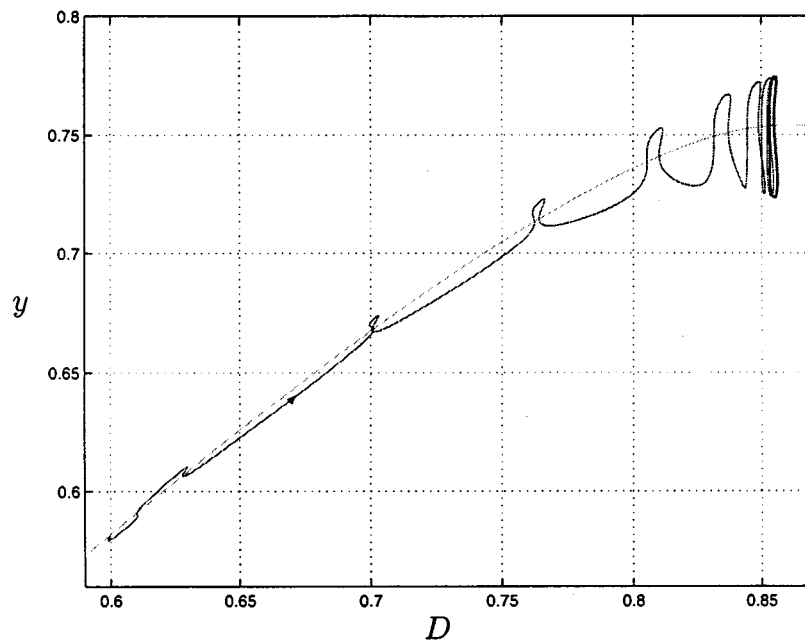
Figure 5. The maximum seeking process for the Monod model with initial dilution rate D_0 = 0.6
