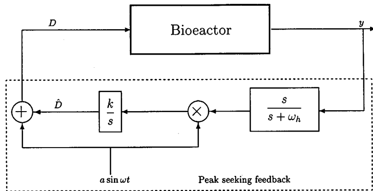
Figure 4. Peak seeking scheme for the bioreactor.
