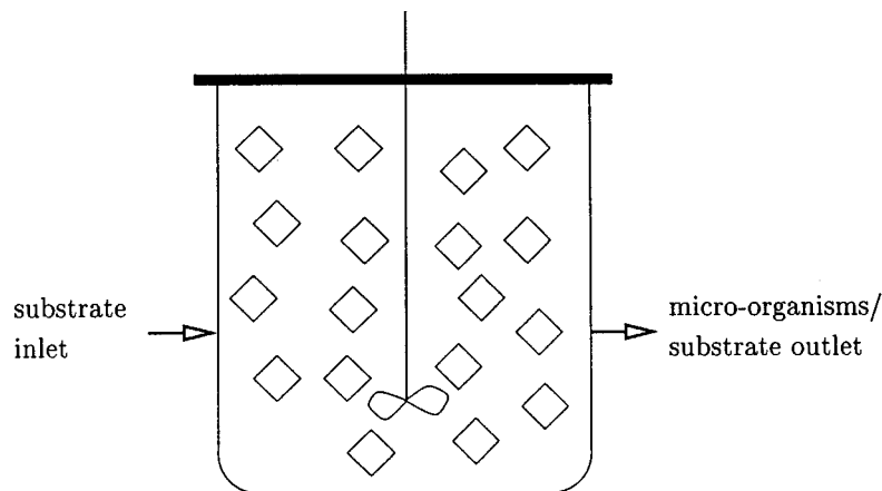
Figure 1. Bioreactor with continuous culture
