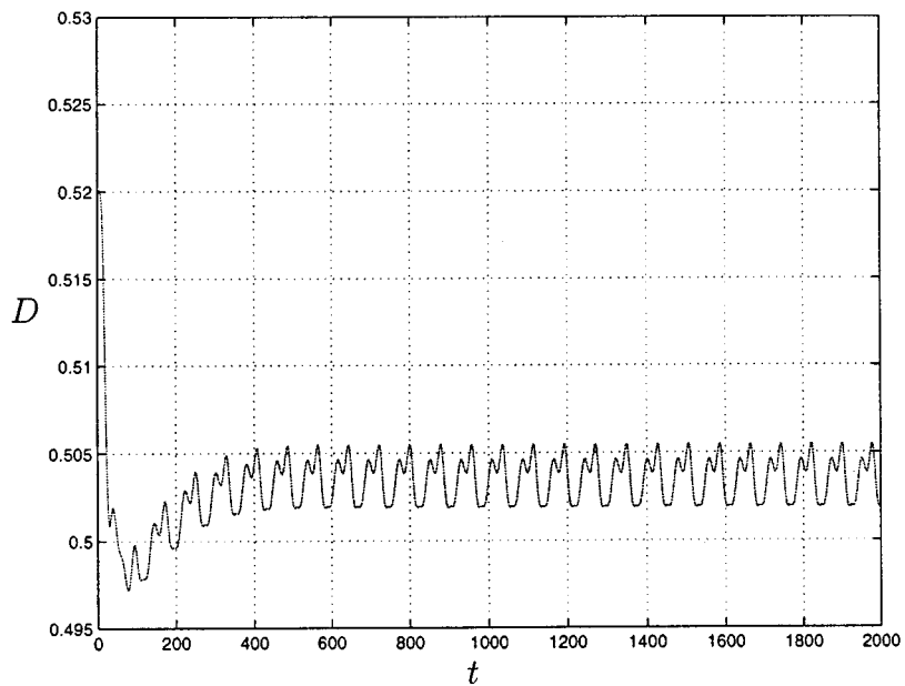
Figure 18. The peak seeking time response of the tuning parameter with state feedback for the Haldane model with initial dilution rate D_0 = 0.52
