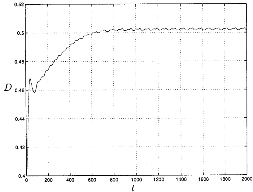
Figure 13. The time response of the tuning parameter with peak seeking for the Haldane model with initial dilution rate D_0 = 0.4
