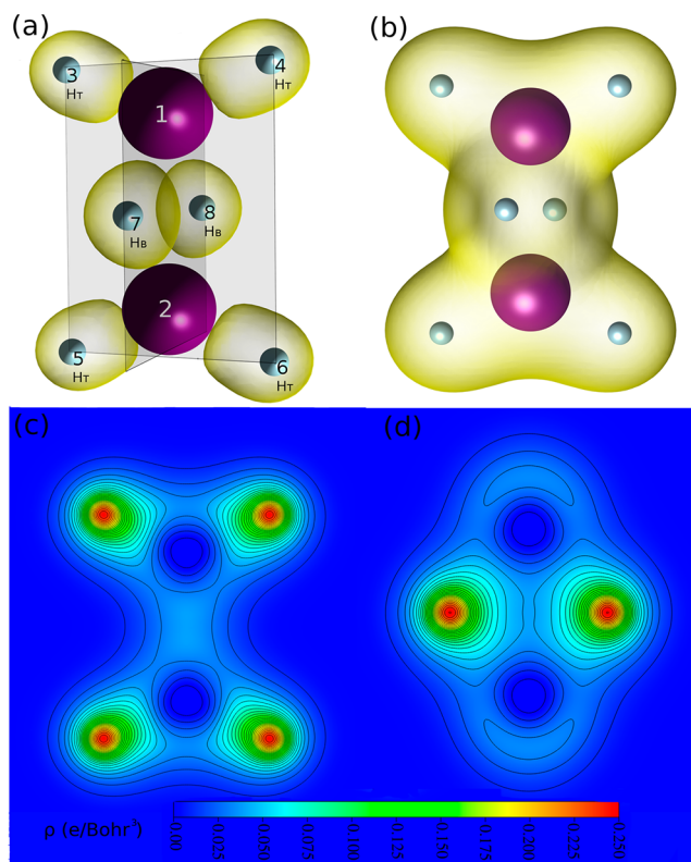
Figure 1. Electronic charge distribution in the digallane molecule ( \text{Ga}_2\text{H}_6 ). (a) Schematic of digallane molecule with an electron density isosurface at 0.042 \text{ e/Bohr}^3 . Atoms 1 and 2 are Ga, while 3 to 8 are H. \text{H}_\text{B} and \text{H}_\text{T} indicate the bridge and terminal atoms of hydrogen, respectively. Atom numbers labeled in this figure correspond to the atom numbers in Table S1, with atoms 1 and 2 replaced by the appropriate group 13 element. Electron density isosurface of digallane at 0.042 \text{ e/Bohr}^3 . (b) Electron density isosurface of digallane at 0.012 \text{ e/Bohr}^3 . (c) Contour maps of valence electron density in the plane that contains atoms 1 to 6 and (d) atoms 1, 2, 7, and 8, which show that Ga atoms transfer charge to the H atoms. Contour lines are at intervals of 0.01 au. Electronic charge distribution for analog molecules can be found in Figure S3.
