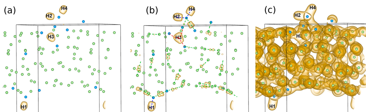
Figure 3. Electron densities of the Ga–H model for a configuration of the MD run at 4400 fs. (a) Isosurfaces at 0.05 \text{ e}^-/\text{Bohr}^3 enclose a small volume only around each of the H atoms. (b) Isosurfaces at 0.04 \text{ e}^-/\text{Bohr}^3 show the electronic density shared in Ga dimers and the H electronic density “pointing” toward neighboring gallium, thus forming bonds similar to the bonds in the molecule digallane. (c) Isosurfaces at 0.03 \text{ e}^-/\text{Bohr}^3 depict electron delocalization throughout the liquid gallium.
