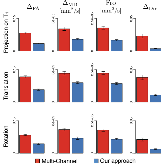
Fig. 5. Estimation of the interpolation errors demonstrates the superiority of the proposed approach compared to the multi-channel alternative to compute linear combinations of multi-fascicle models. The bar plots show the interpolation error for four metrics ( \Delta_{FA} , \Delta_{MD} , Fro and \Delta_{Dir} ) under three different transformations.
