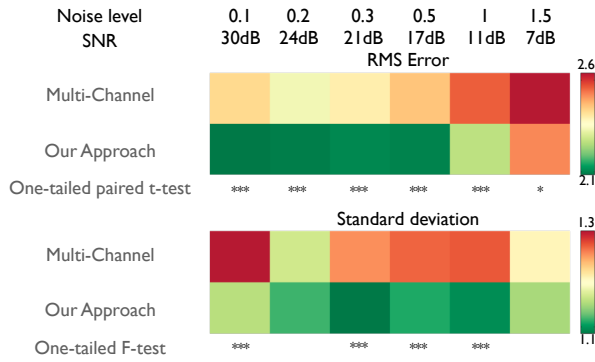
Fig. 9. Our mathematical framework leads to higher registration accuracies than the multi-channel alternative: the RMS errors (top) and its variance (bottom) are significantly lower. Results are shown for 1,440 registrations performed at various SNR for synthetic deformation fields (* p < 0.05 , ** p < 0.005 , *** p < 0.001 ).
