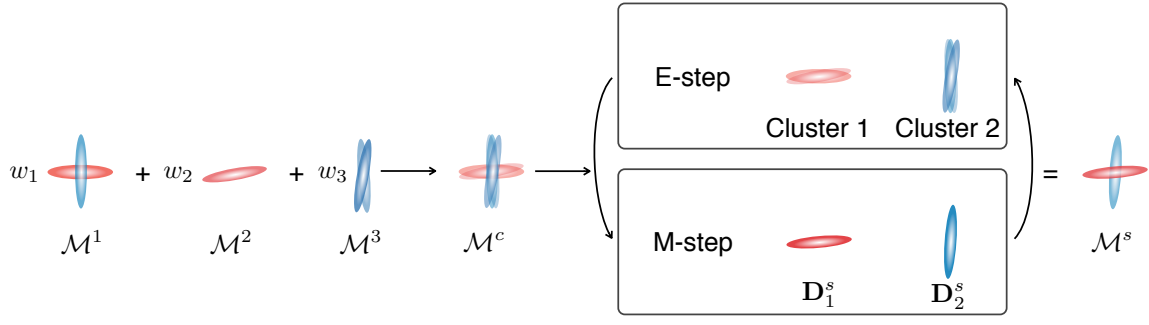
Fig. 1. Computing weighted combinations of multi-fascicle models amounts to computing the complete mixture \mathcal{M}^c and simplifying it in an EM scheme to obtain \mathcal{M}^s . The E-step is a clustering problem and the M-step consists in averaging log-tensors in each cluster.
