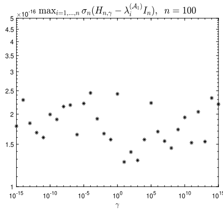
Fig. 9. \max_{i=1,\dots,n} \sigma_n(H_{n,\gamma} - \lambda_i^{(A_1)} I_n) , \gamma = 10^{-k} , k = -15, -14, \dots, -1, 0, 1, \dots, 14, 15 , n = 100 .
