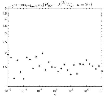
Fig. 10. \max_{i=1,\dots,n} \sigma_n(H_{n,\gamma} - \lambda_i^{(A_1)} I_n) , \gamma = 10^{-k} , k = -15, -14, \dots, -1, 0, 1, \dots, 14, 15 , n = 200 .
