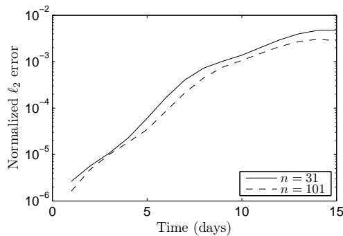
Fig. 14. A time series of the error measured against the DG reference solution for the Rossby-Haurwitz test case, with N = 25,600 .
