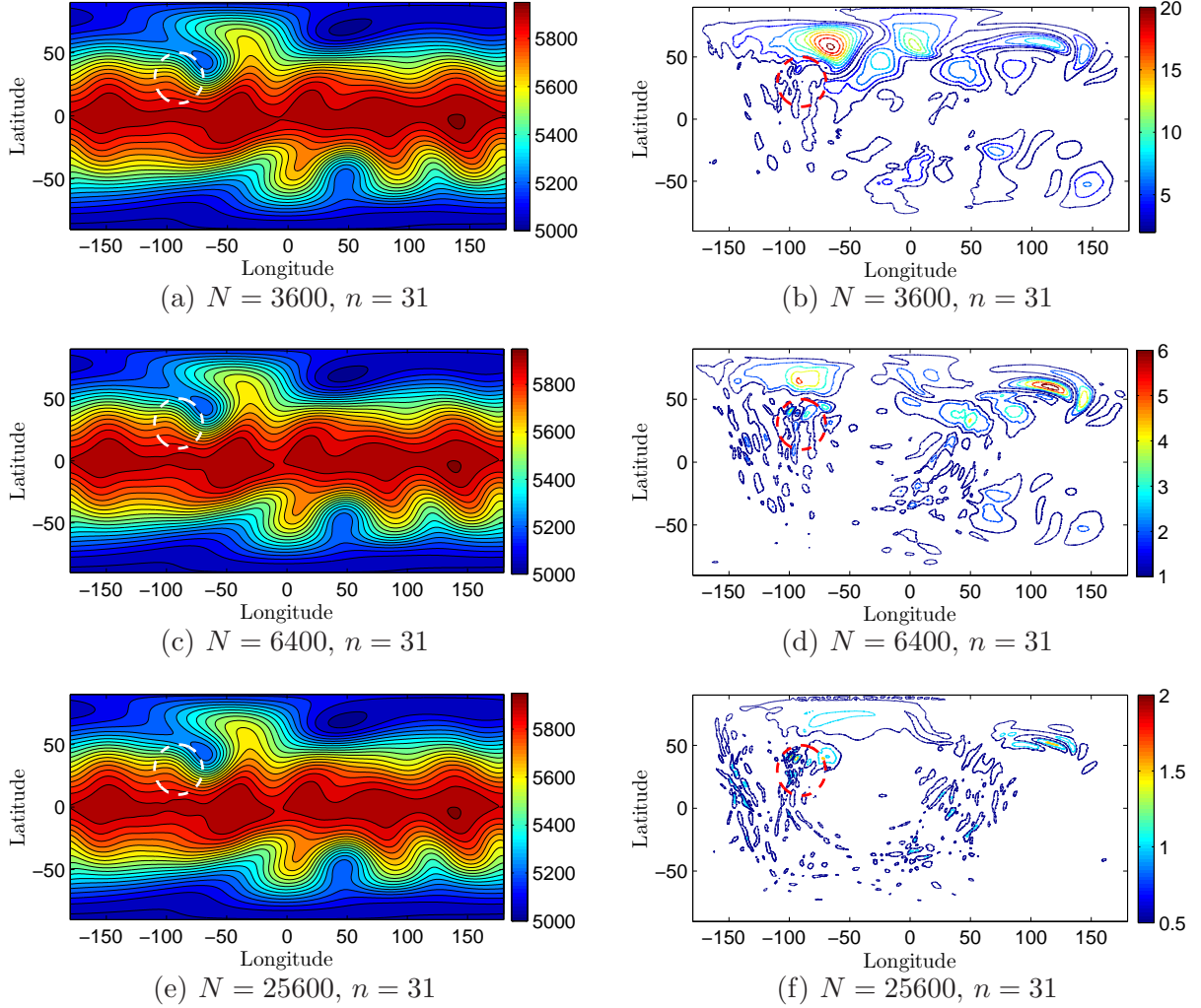
Fig. 7. Left column: The height field h for flow over a conical mountain at day 15 for varying N with n = 31 . Contour interval is 50m. Right column: Magnitude of the error between the RBF-FD solution and the DG reference solution. Contour interval for N=3600 is 2m, for N=6400 is 1m, and for N=25,600 is 0.5m.
