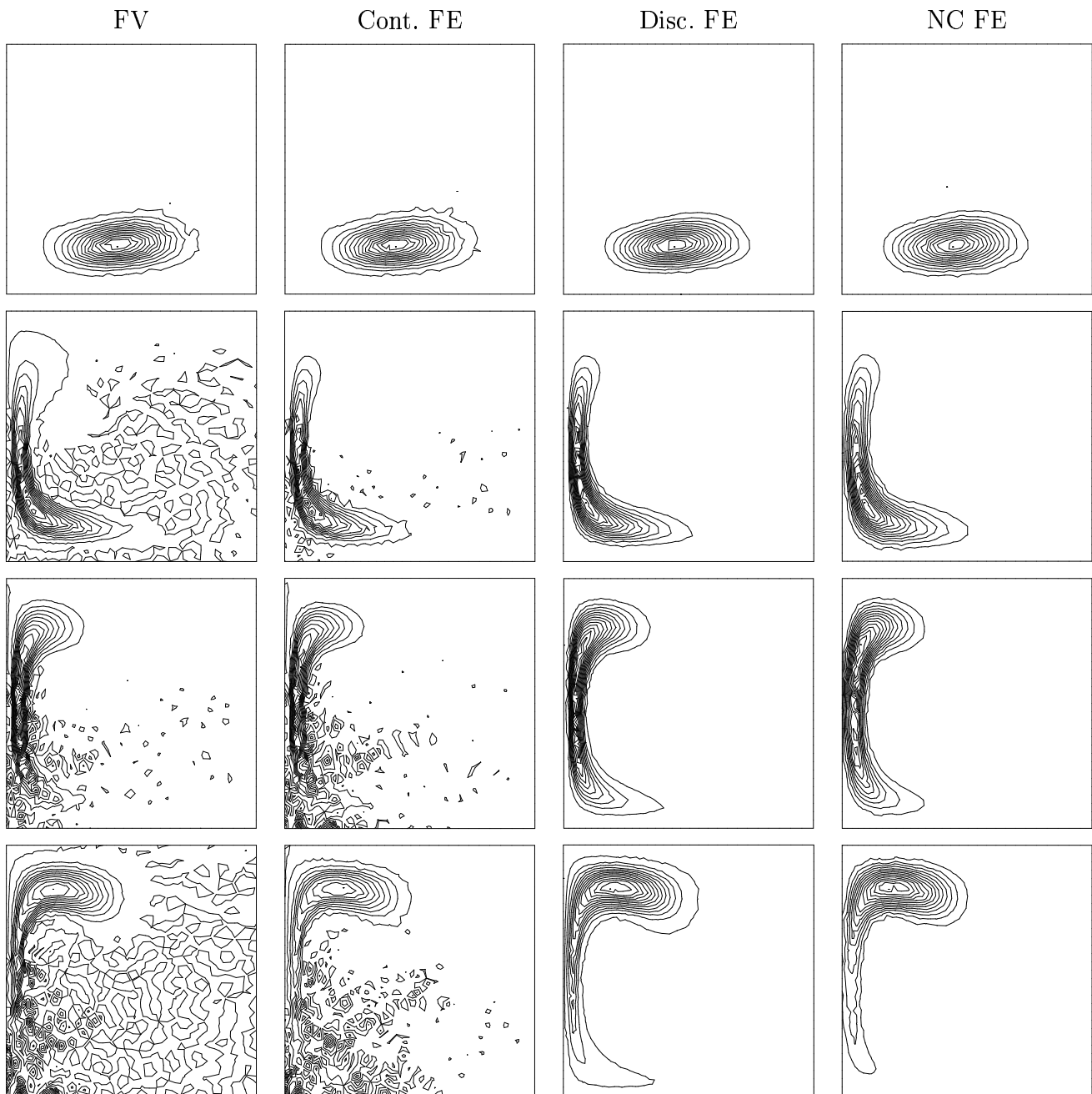
Figure 9. Snapshots of the simulated tracer field after 2 \times 10^6 , 4 \times 10^6 , 5 \times 10^6 and 6 \times 10^6 seconds respectively for pure advection with the finite volume (FV), continuous finite element (Cont. FE), discontinuous finite element (Disc. FE) and non-conforming finite element (NC FE) schemes. There are 13 isolines.
