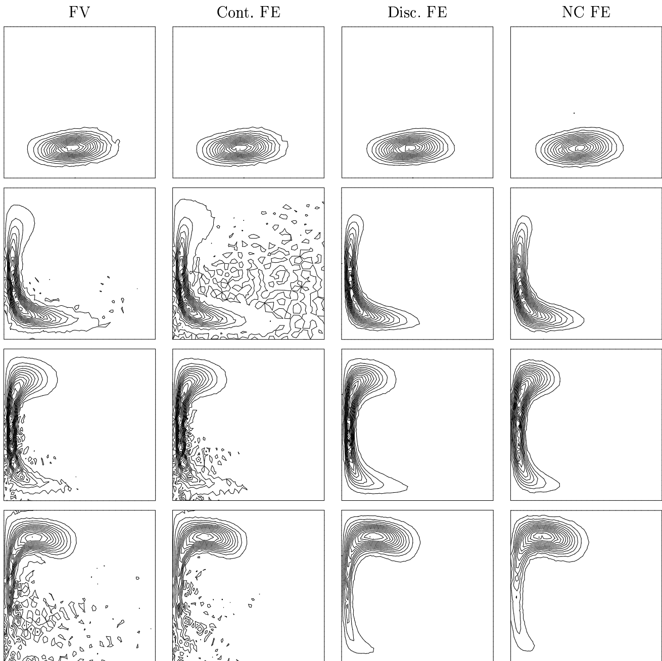
Figure 11. Snapshots of the simulated tracer field after 2 \times 10^6 , 4 \times 10^6 , 5 \times 10^6 and 6 \times 10^6 seconds respectively for advection-diffusion ( K = 30 \text{ m}^2/\text{s} ) with the finite volume, continuous finite element, discontinuous finite element and non-conforming finite element schemes. There are 13 isolines.
