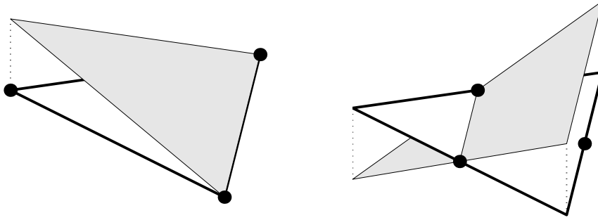
Figure 3. Shape functions (in grey) associated with continuous and discontinuous approximations (left) and non-conforming approximations (right).
