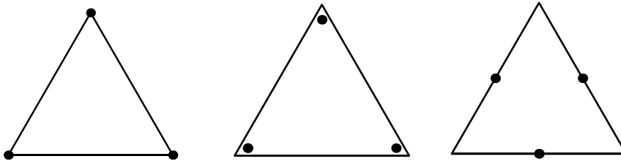
Figure 4. Nodal values ( \bullet ) distributions for the linear continuous (left), discontinuous (centre) and non-conforming (right) approximations.
