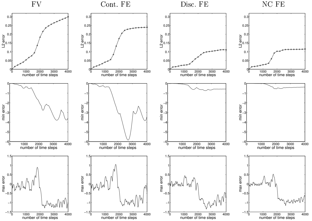
Figure 10. L_2 (top), min (middle) and max (bottom) errors resulting from pure advection of the tracer profile.
