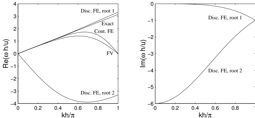
Figure 6. Dispersion relations of the discontinuous finite element (Disc. FE), continuous finite element (Cont. FE) and finite volume (FV) schemes compared to the exact relation. The left and right panels represent the real and imaginary parts of the dispersion relation respectively.
