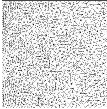
Figure 7. Unstructured mesh used for the gaussian hill transport simulation. This mesh has 2222 elements and there are approximately 5 elements in the boundary layer.
