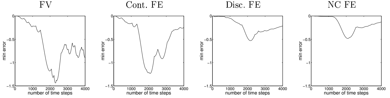
Figure 12. min errors resulting from advection-diffusion of the tracer profile.
