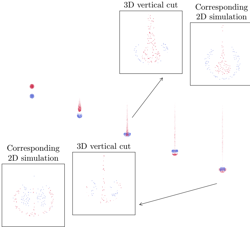
Fig. 4: Shape evolution of vertically aligned interacting clouds using the parameter Set 2 in Table 1. Clouds states are shifted to the right each time interval of \Delta t = 12.5s .
